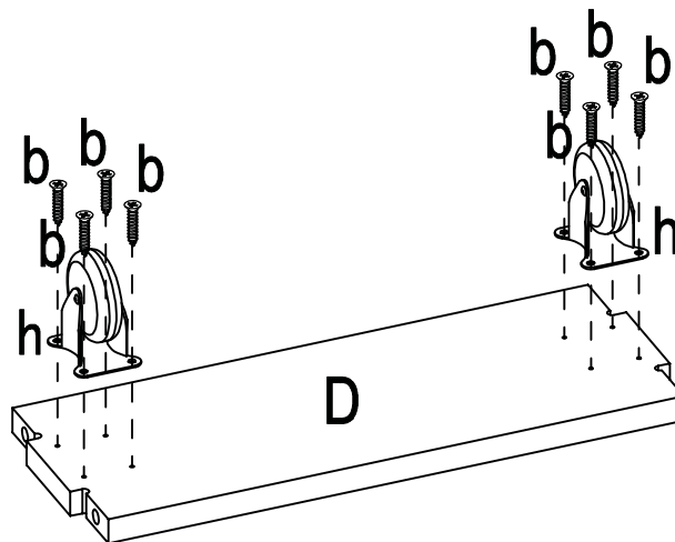
Unit-2 2 pcs
