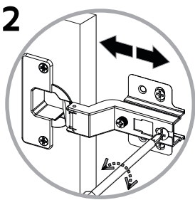
Depth adjustment
