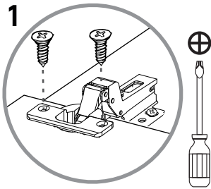
Hinge adjustment
