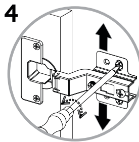
Height adjustment
