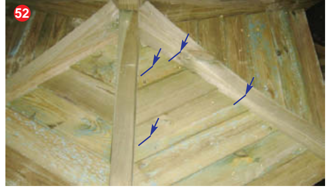
52 Secure roof panels to the top roof rafters using 4 x 50mm screws per panel.
